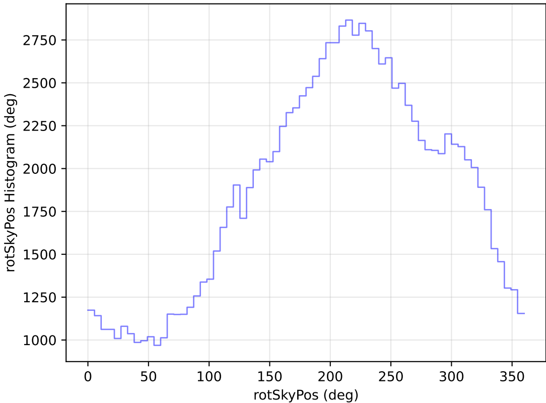
too_elab_r64_d2_giz_v3.4_10yrs All sky u band: rotSkyPos Histogram
