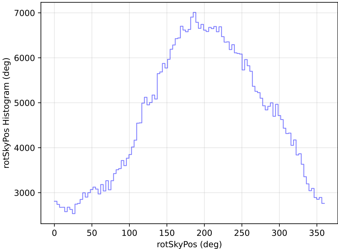
too_elab_r64_d2_giz_v3.4_10yrs All sky r band: rotSkyPos Histogram
