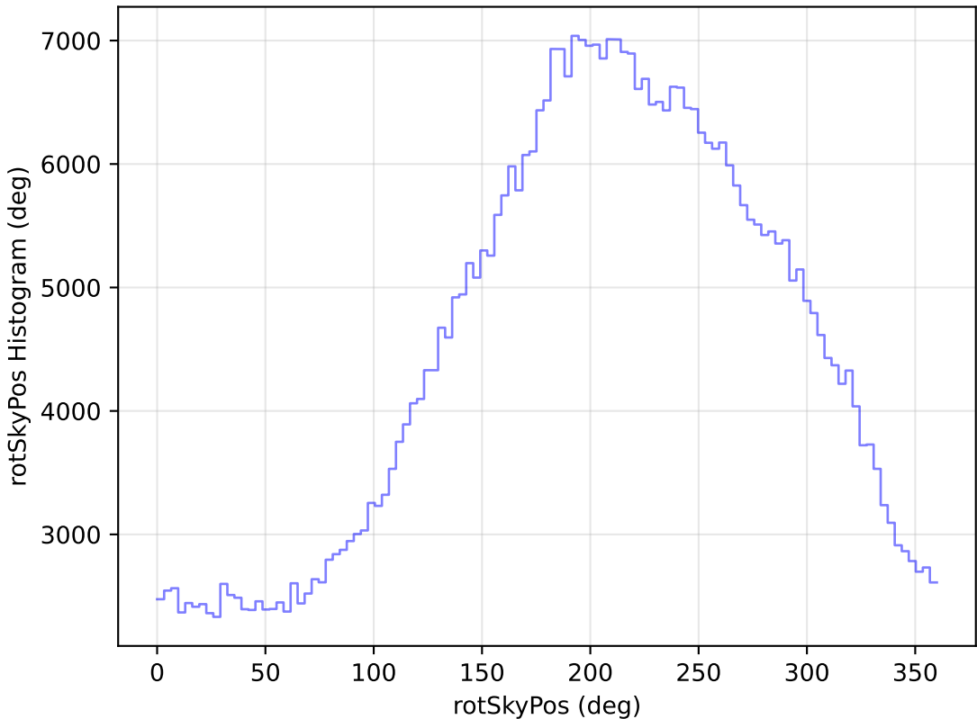
too_elab_r64_d2_giz_v3.4_10yrs All sky i band: rotSkyPos Histogram
