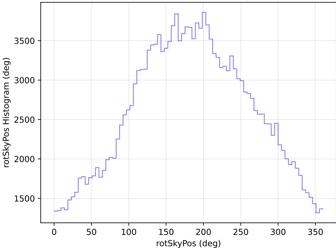
too_elab_r64_d2_giz_v3.4_10yrs All sky g band: rotSkyPos Histogram
