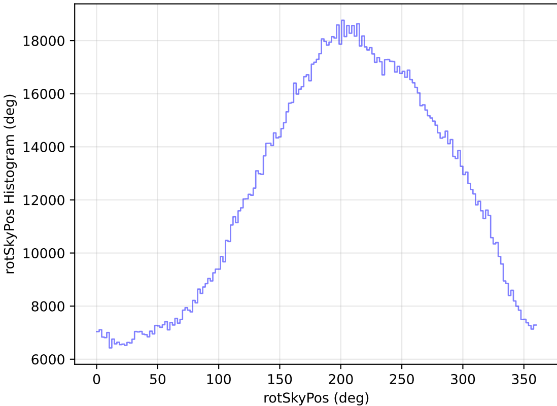
too_elab_r64_d2_giz_v3.4_10yrs All sky all bands: rotSkyPos Histogram
