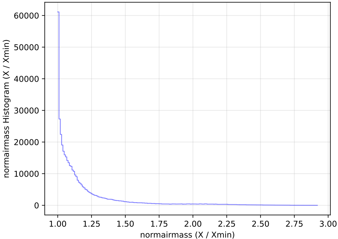
too_elab_r64_d2_giz_v3.4_10yrs WFD z band: normairmass Histogram
