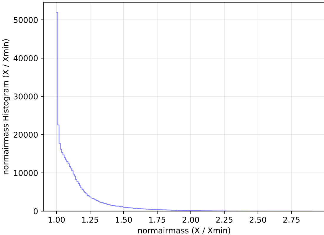
too_elab_r64_d2_giz_v3.4_10yrs WFD y band: normairmass Histogram
