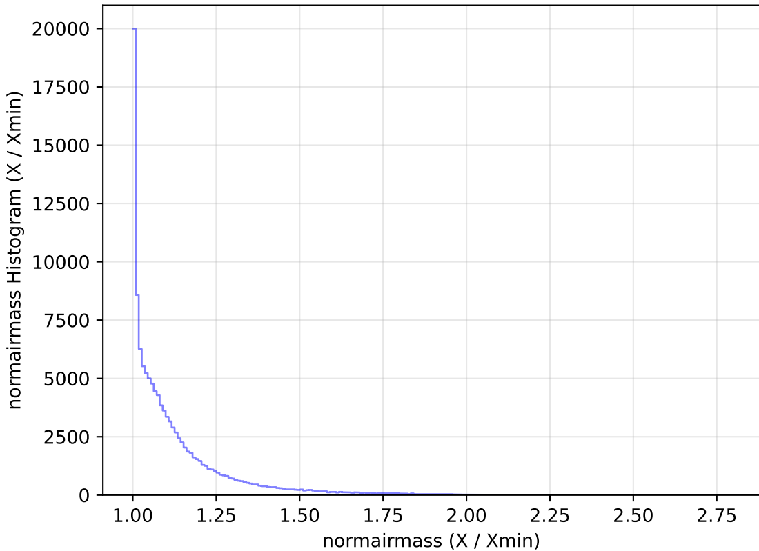
too_elab_r64_d2_giz_v3.4_10yrs WFD u band: normairmass Histogram
