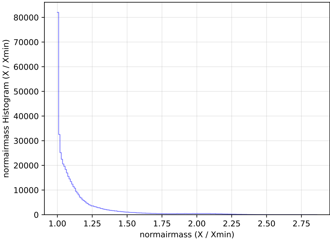
too_elab_r64_d2_giz_v3.4_10yrs WFD r band: normairmass Histogram
