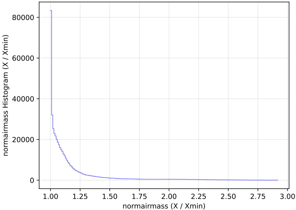
too_elab_r64_d2_giz_v3.4_10yrs WFD i band: normairmass Histogram
