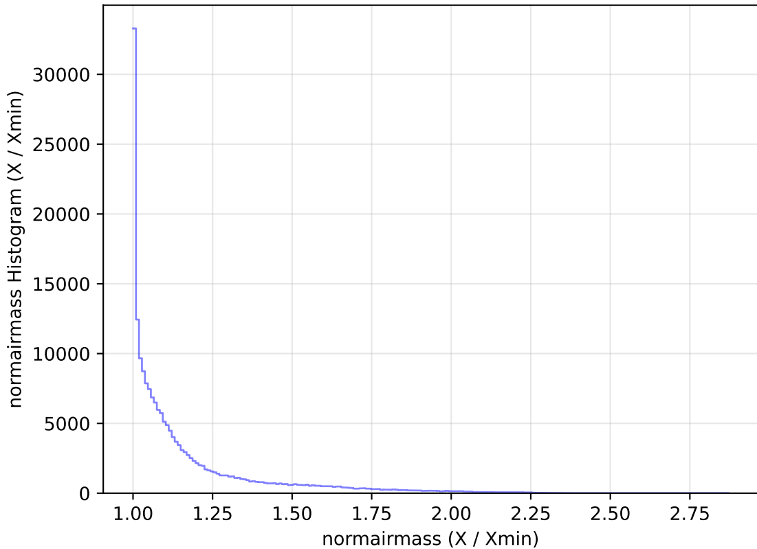
too_elab_r64_d2_giz_v3.4_10yrs WFD g band: normairmass Histogram
