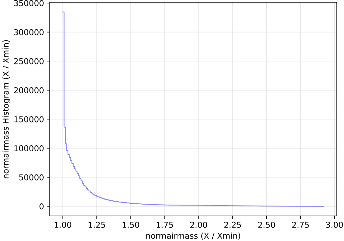
too_elab_r64_d2_giz_v3.4_10yrs WFD all bands: normairmass Histogram
