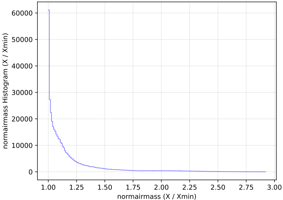
too_elab_r64_d2_giz_v3.4_10yrs All sky z band: normairmass Histogram
