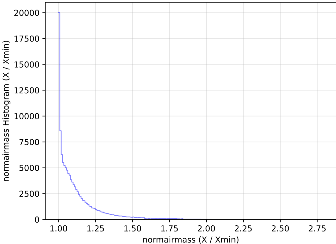
too_elab_r64_d2_giz_v3.4_10yrs All sky u band: normairmass Histogram
