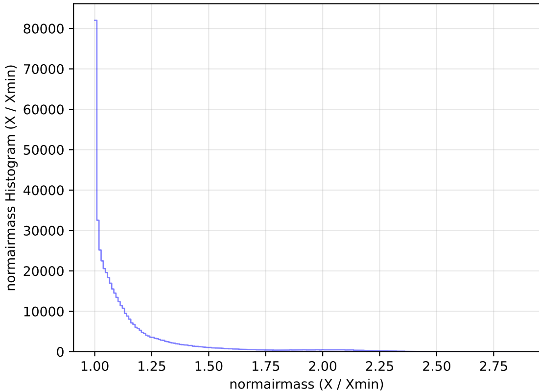
too_elab_r64_d2_giz_v3.4_10yrs All sky r band: normairmass Histogram
