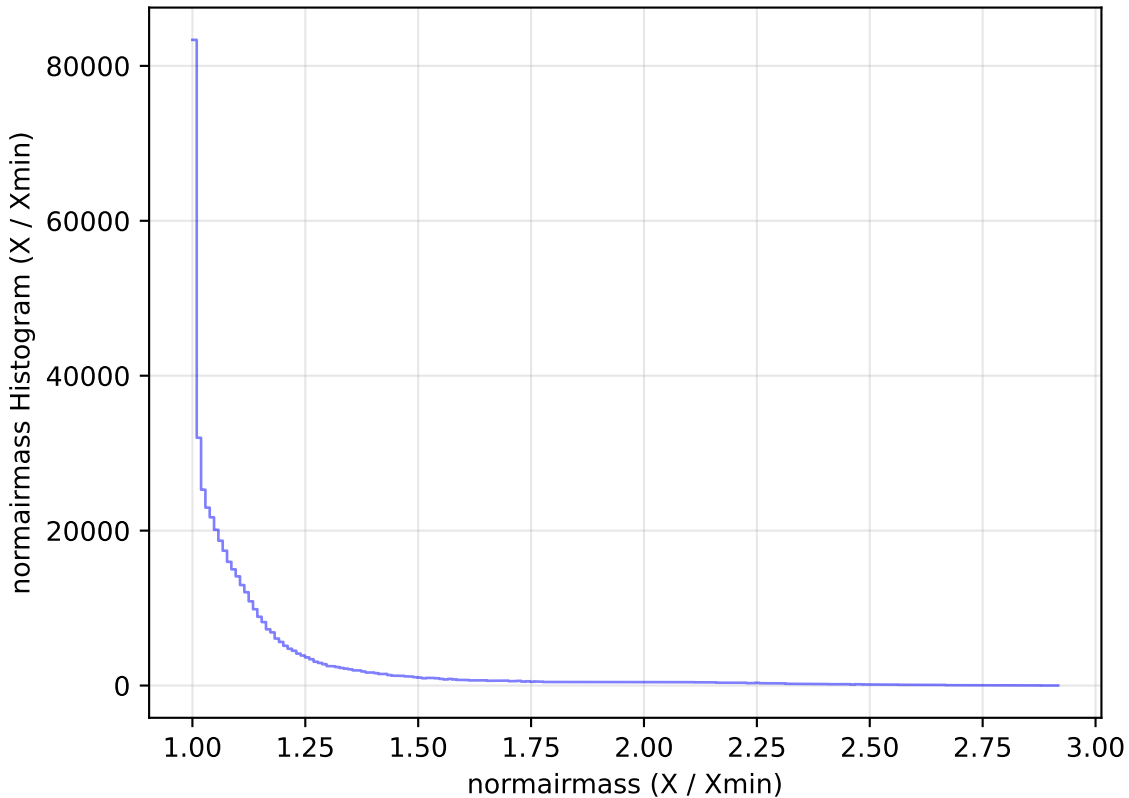
too_elab_r64_d2_giz_v3.4_10yrs All sky i band: normairmass Histogram
