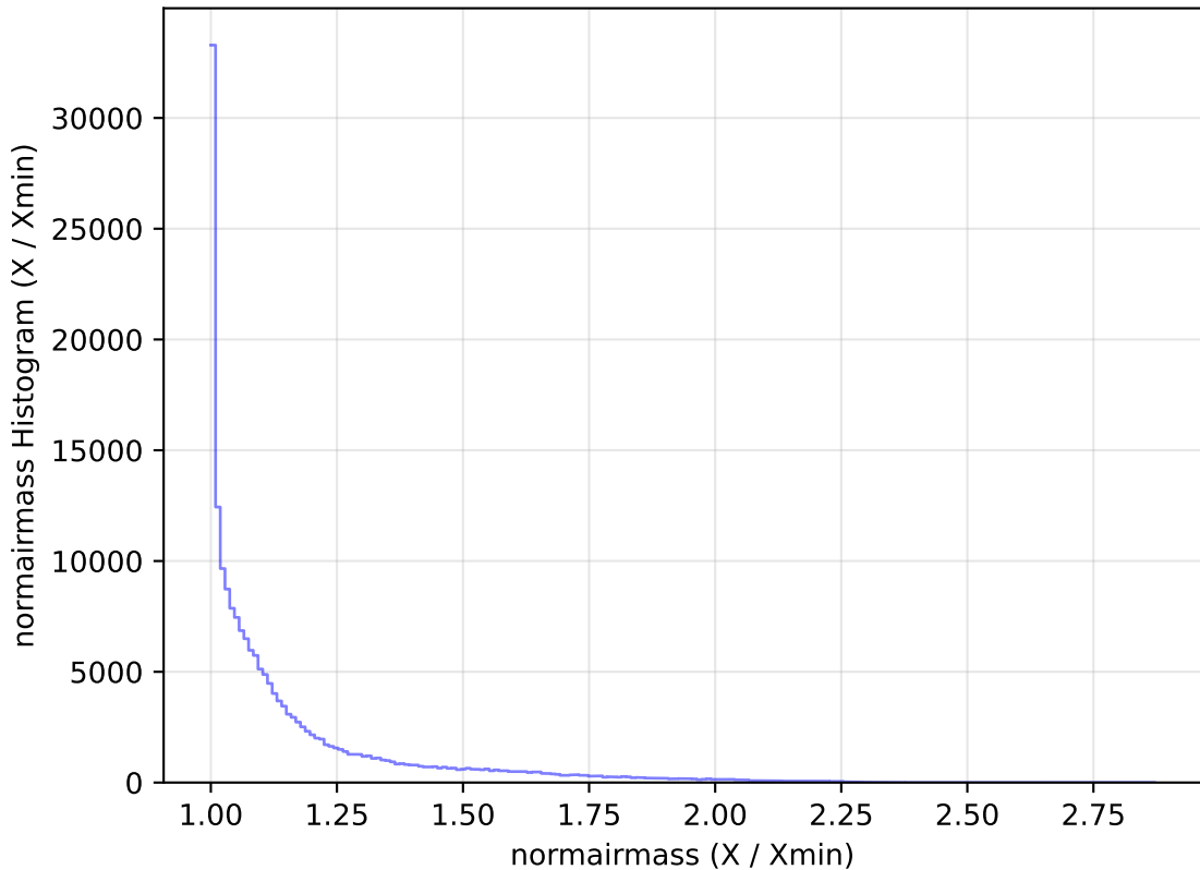
too_elab_r64_d2_giz_v3.4_10yrs All sky g band: normairmass Histogram
