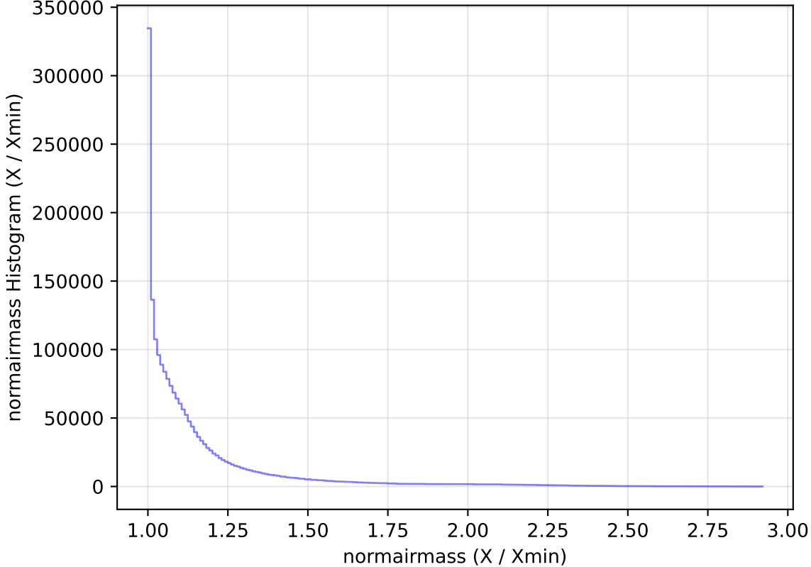
too_elab_r64_d2_giz_v3.4_10yrs All sky all bands: normairmass Histogram
