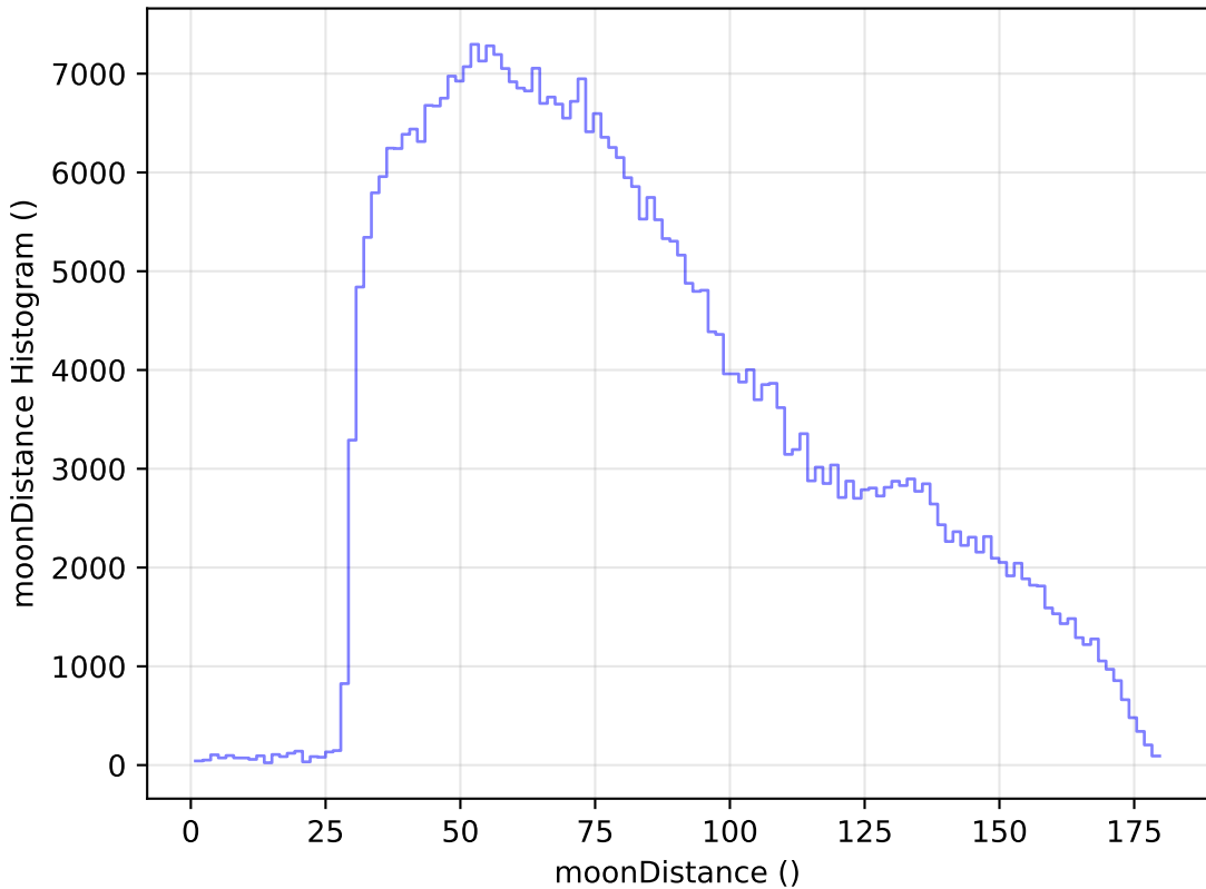
too_elab_r64_d2_giz_v3.4_10yrs WFD z band: moonDistance Histogram
