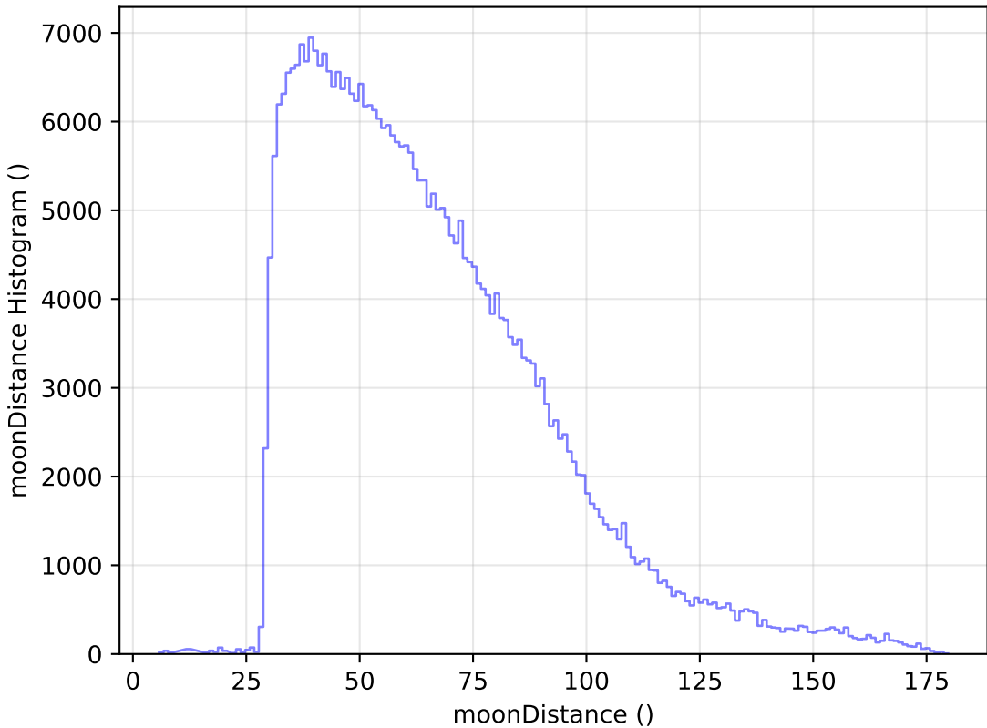
too_elab_r64_d2_giz_v3.4_10yrs WFD y band: moonDistance Histogram
