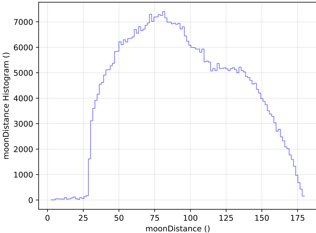
too_elab_r64_d2_giz_v3.4_10yrs WFD i band: moonDistance Histogram
