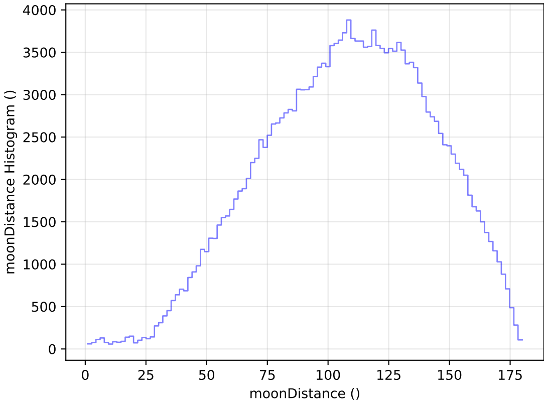
too_elab_r64_d2_giz_v3.4_10yrs WFD g band: moonDistance Histogram
