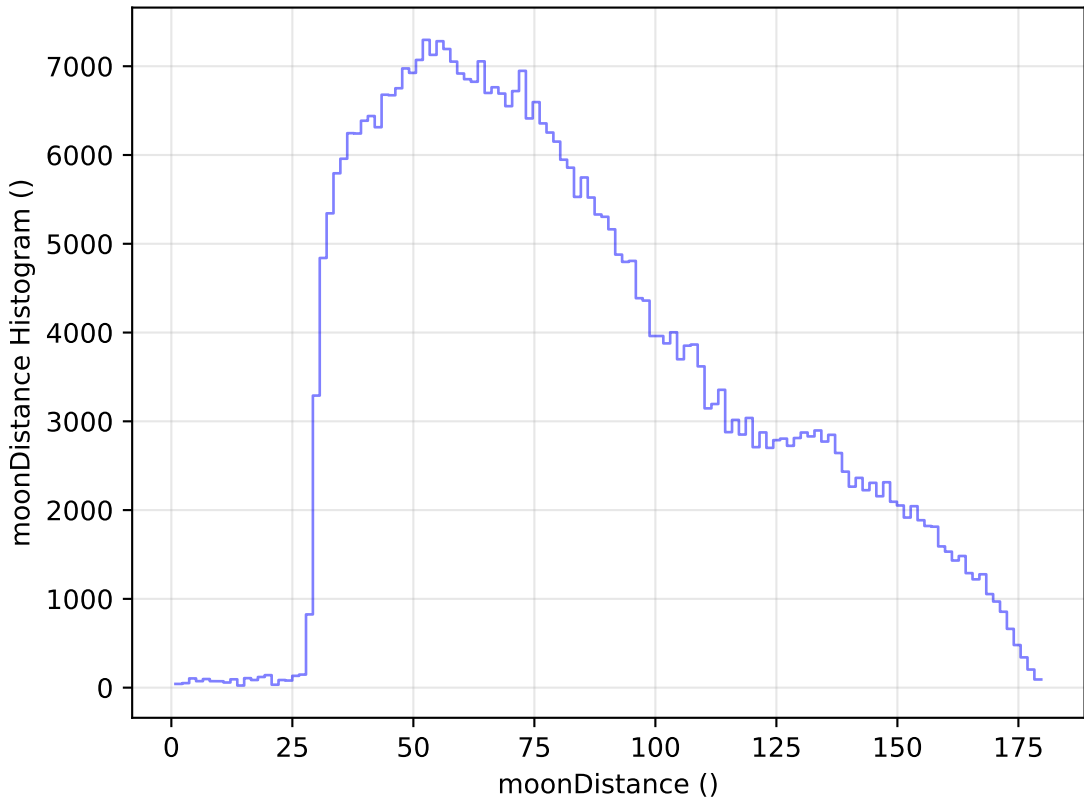
too_elab_r64_d2_giz_v3.4_10yrs All sky z band: moonDistance Histogram
