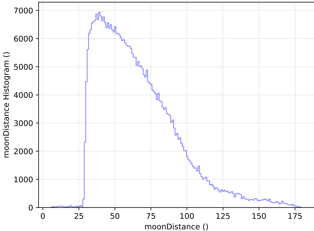
too_elab_r64_d2_giz_v3.4_10yrs All sky y band: moonDistance Histogram
