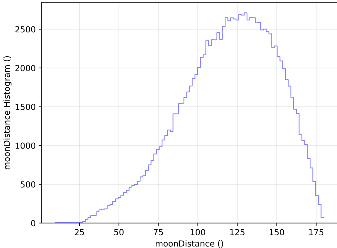
too_elab_r64_d2_giz_v3.4_10yrs All sky u band: moonDistance Histogram
