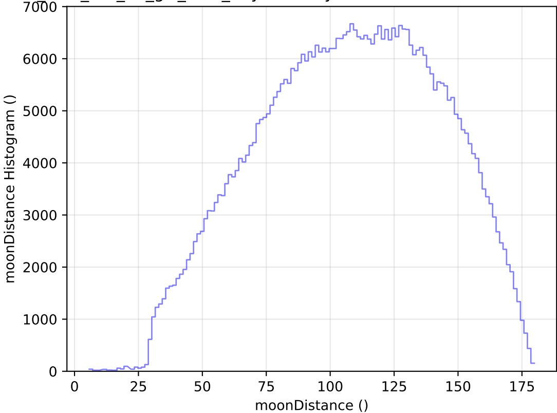
too_elab_r64_d2_giz_v3.4_10yrs All sky r band: moonDistance Histogram
