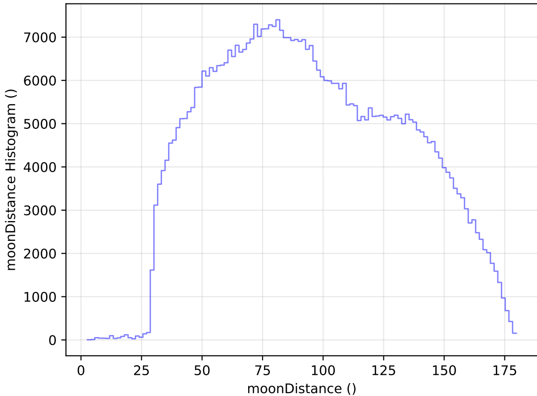
too_elab_r64_d2_giz_v3.4_10yrs All sky i band: moonDistance Histogram
