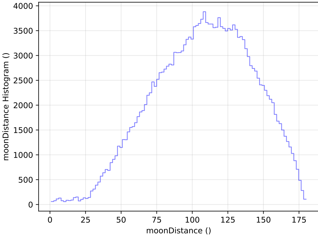
too_elab_r64_d2_giz_v3.4_10yrs All sky g band: moonDistance Histogram
