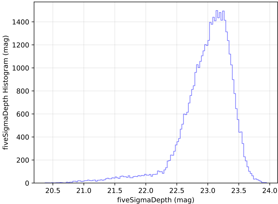
too_elab_r64_d2_giz_v3.4_10yrs Yr 1 z band: fiveSigmaDepth Histogram
