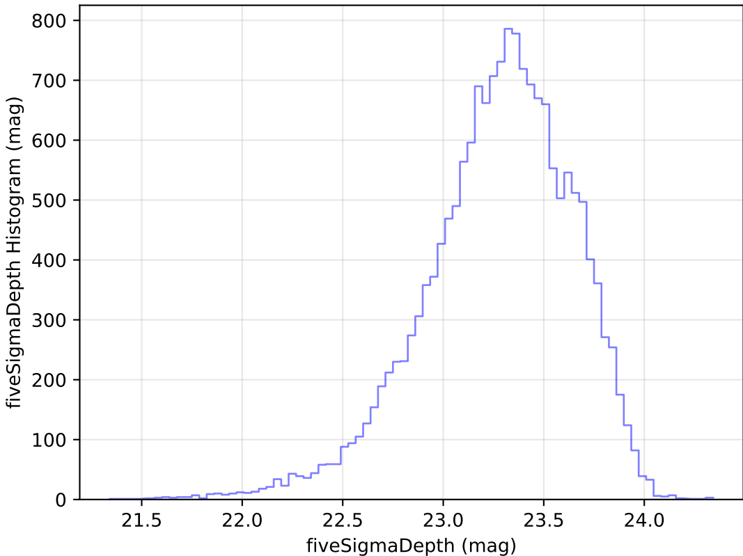
too_elab_r64_d2_giz_v3.4_10yrs Yr 1 u band: fiveSigmaDepth Histogram
