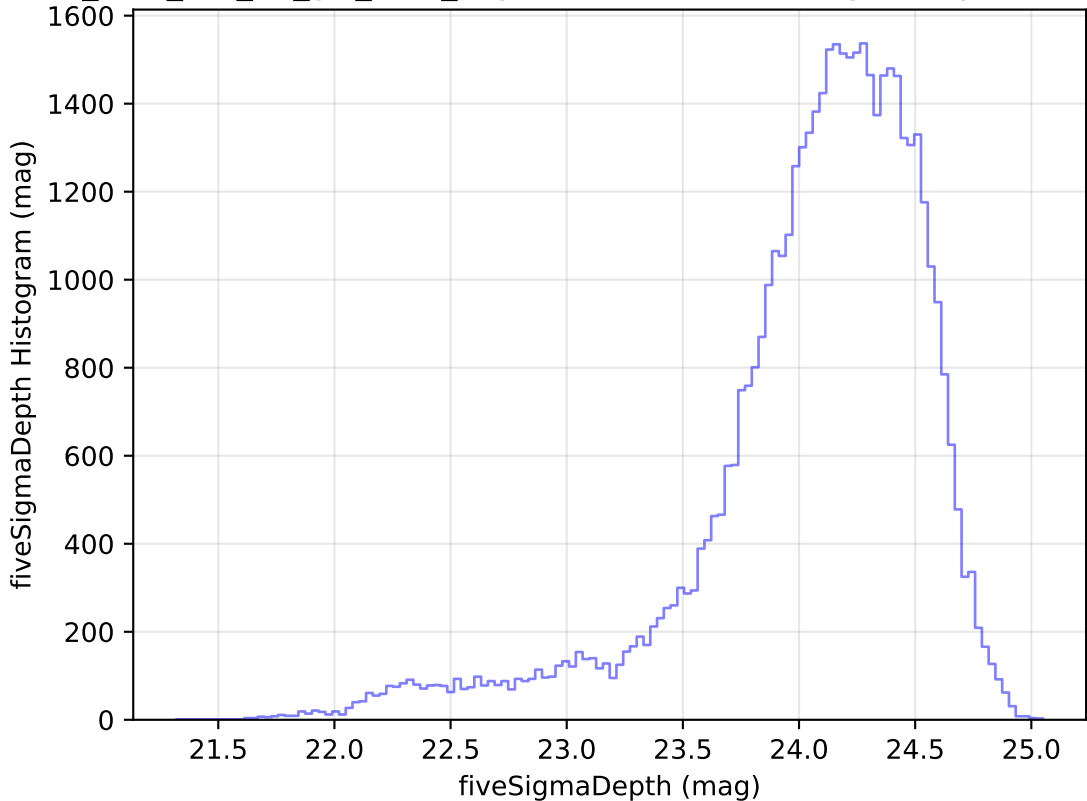
too_elab_r64_d2_giz_v3.4_10yrs Yr 1 r band: fiveSigmaDepth Histogram
