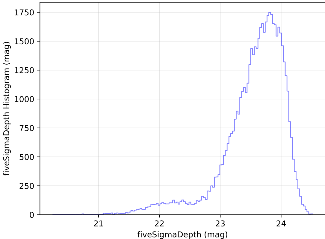
too_elab_r64_d2_giz_v3.4_10yrs Yr 1 i band: fiveSigmaDepth Histogram
