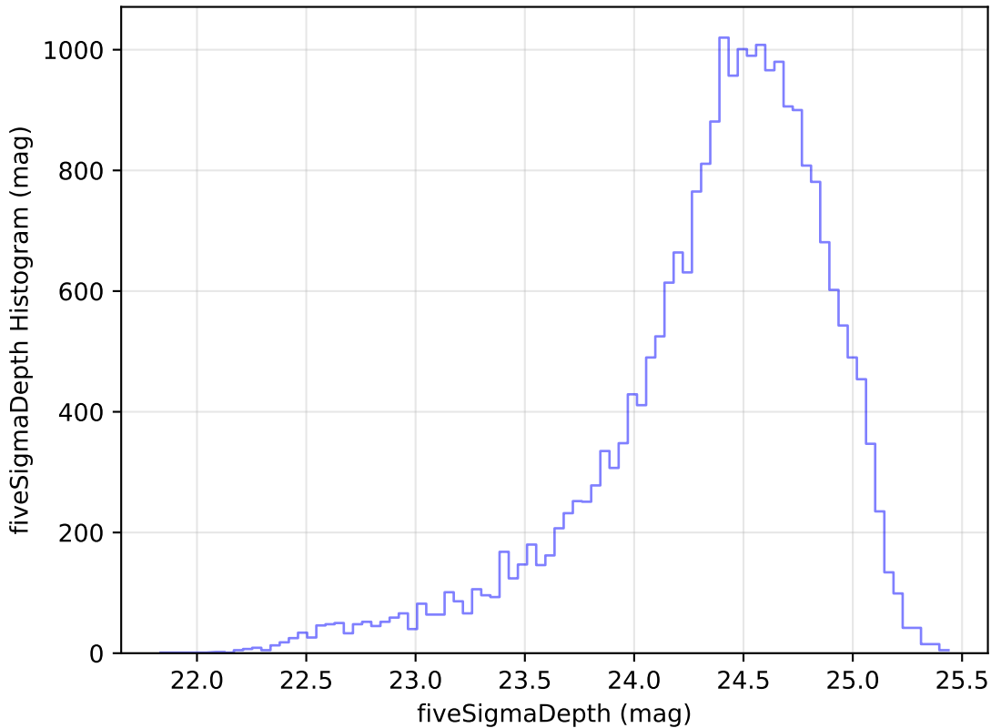
too_elab_r64_d2_giz_v3.4_10yrs Yr 1 g band: fiveSigmaDepth Histogram
