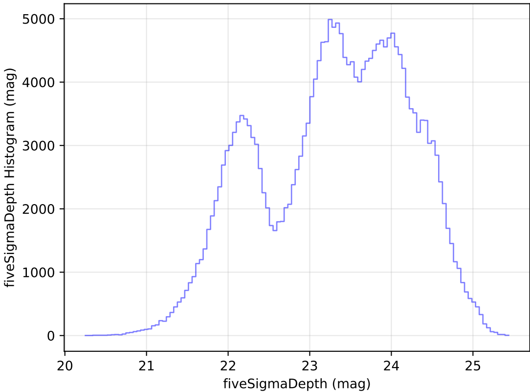
too_elab_r64_d2_giz_v3.4_10yrs Yr 1 all bands: fiveSigmaDepth Histogram
