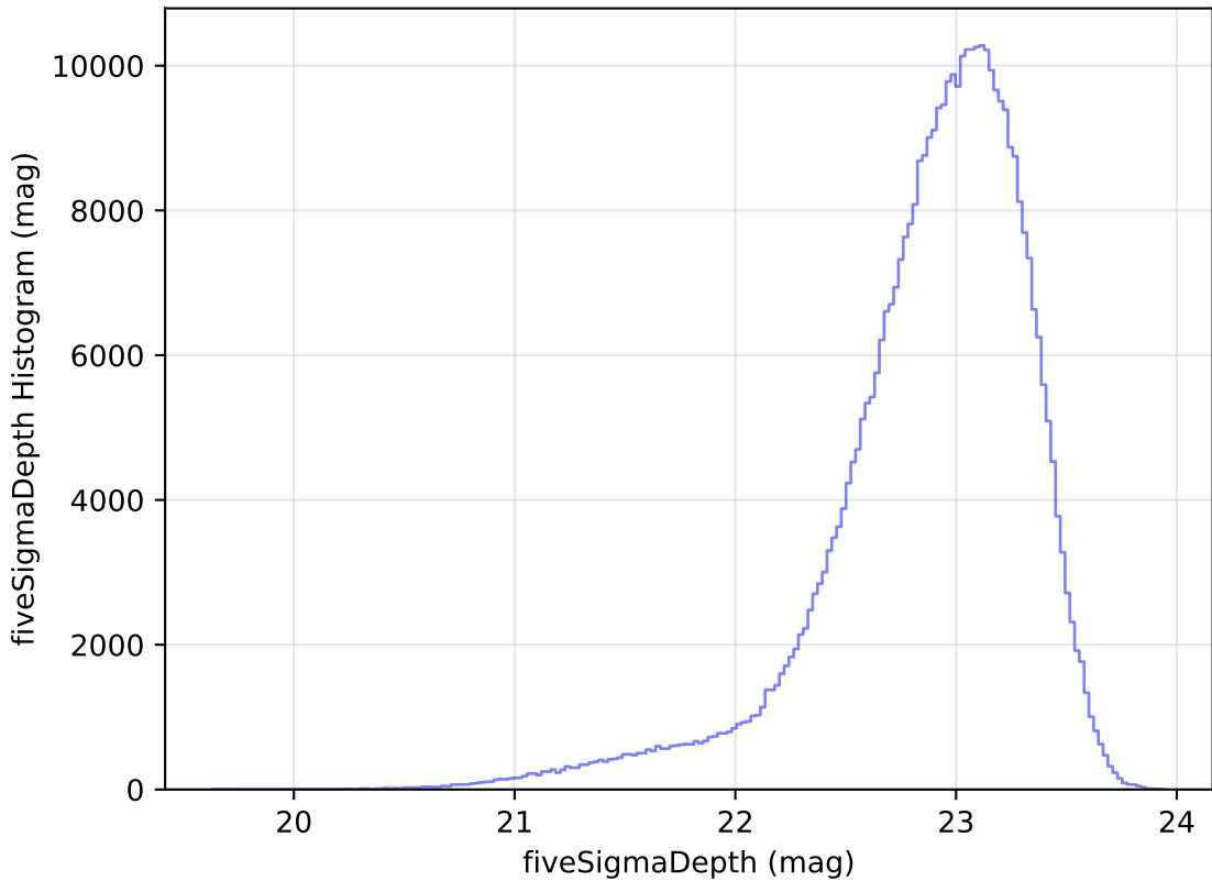
too_elab_r64_d2_giz_v3.4_10yrs WFD z band: fiveSigmaDepth Histogram
