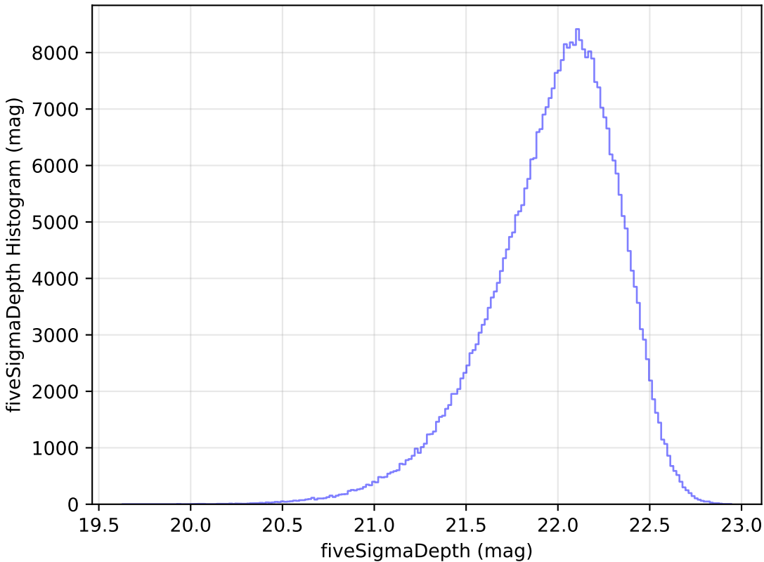
too_elab_r64_d2_giz_v3.4_10yrs WFD y band: fiveSigmaDepth Histogram
