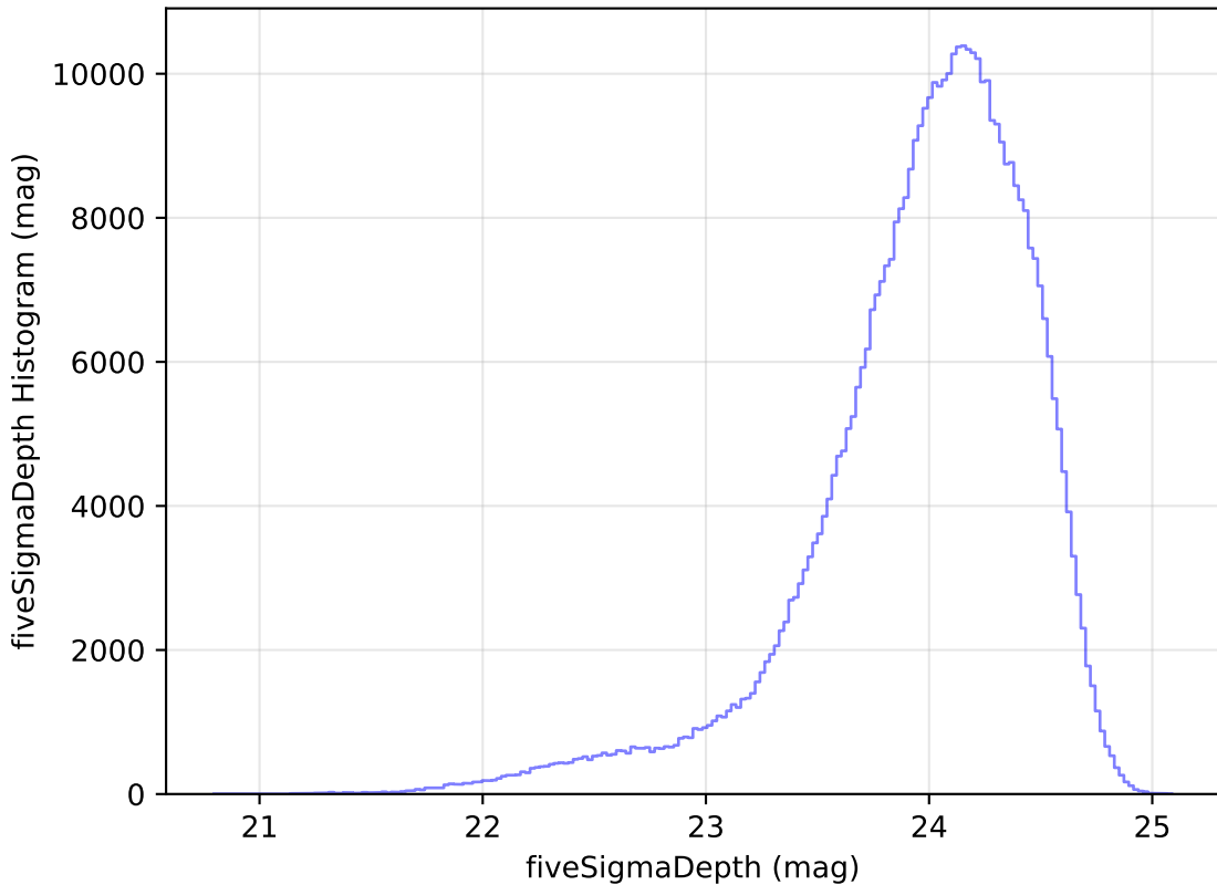
too_elab_r64_d2_giz_v3.4_10yrs WFD r band: fiveSigmaDepth Histogram
