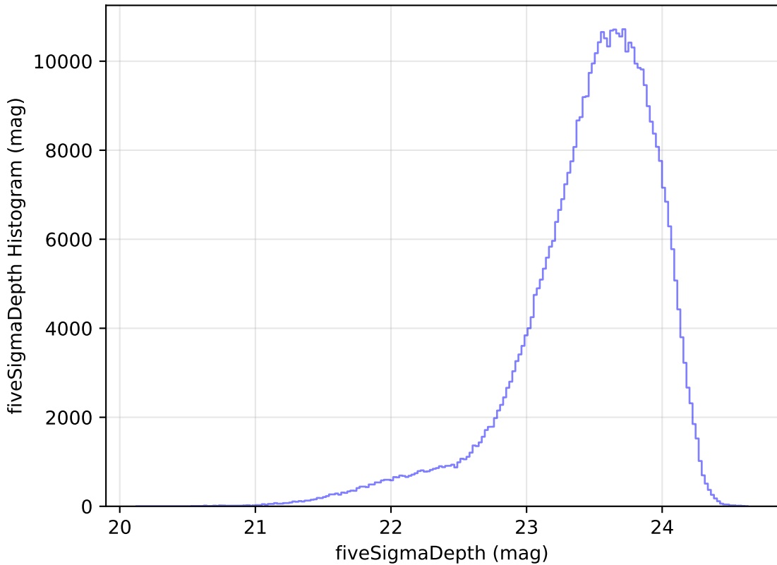
too_elab_r64_d2_giz_v3.4_10yrs WFD i band: fiveSigmaDepth Histogram
