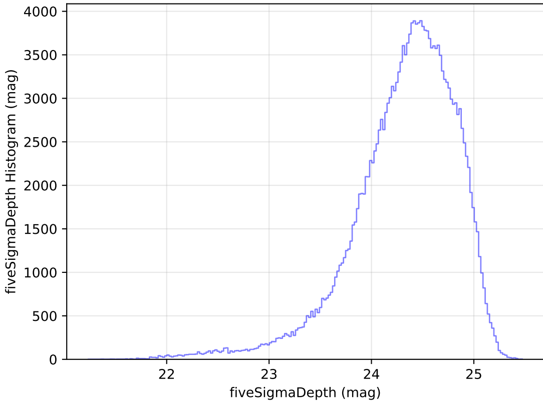
too_elab_r64_d2_giz_v3.4_10yrs WFD g band: fiveSigmaDepth Histogram
