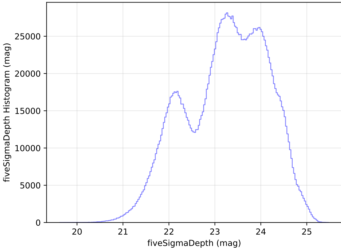
too_elab_r64_d2_giz_v3.4_10yrs WFD all bands: fiveSigmaDepth Histogram
