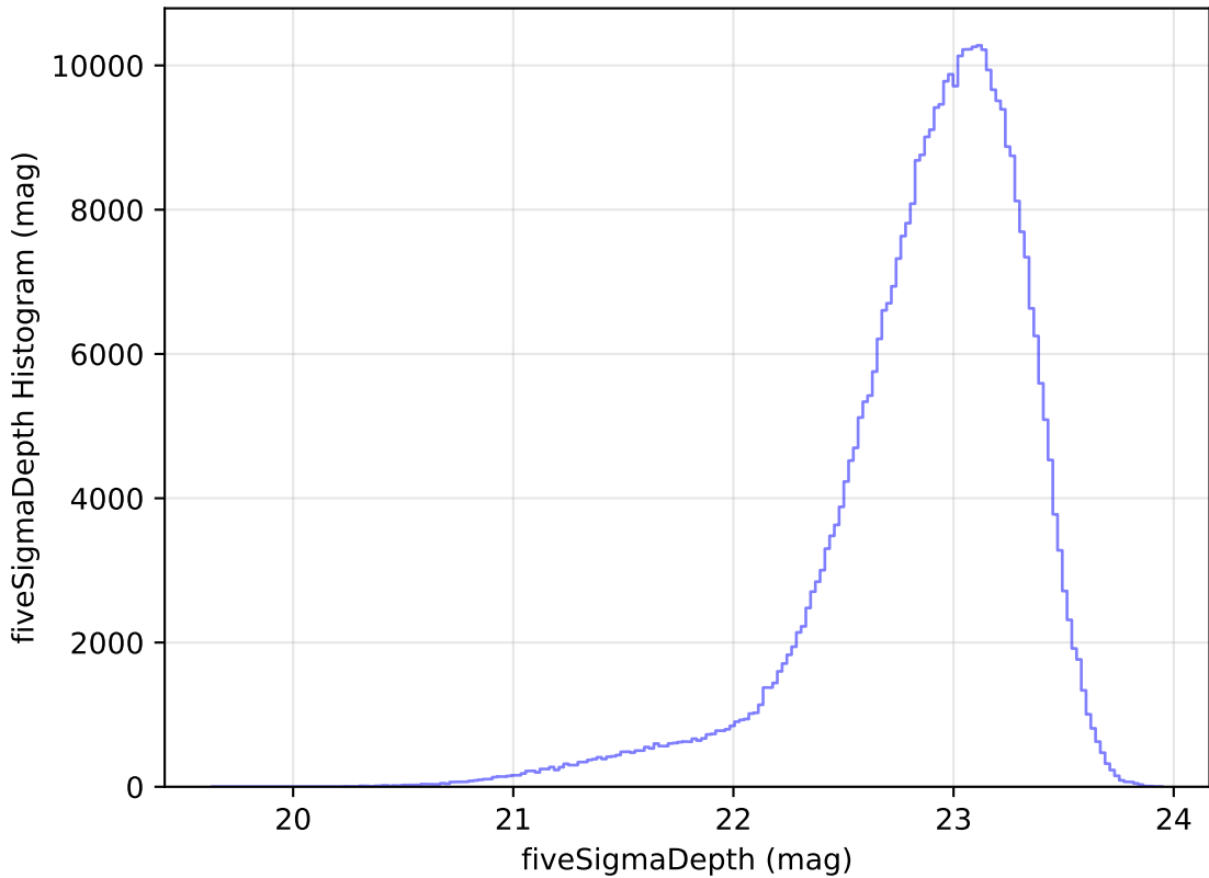
too_elab_r64_d2_giz_v3.4_10yrs All sky z band: fiveSigmaDepth Histogram
