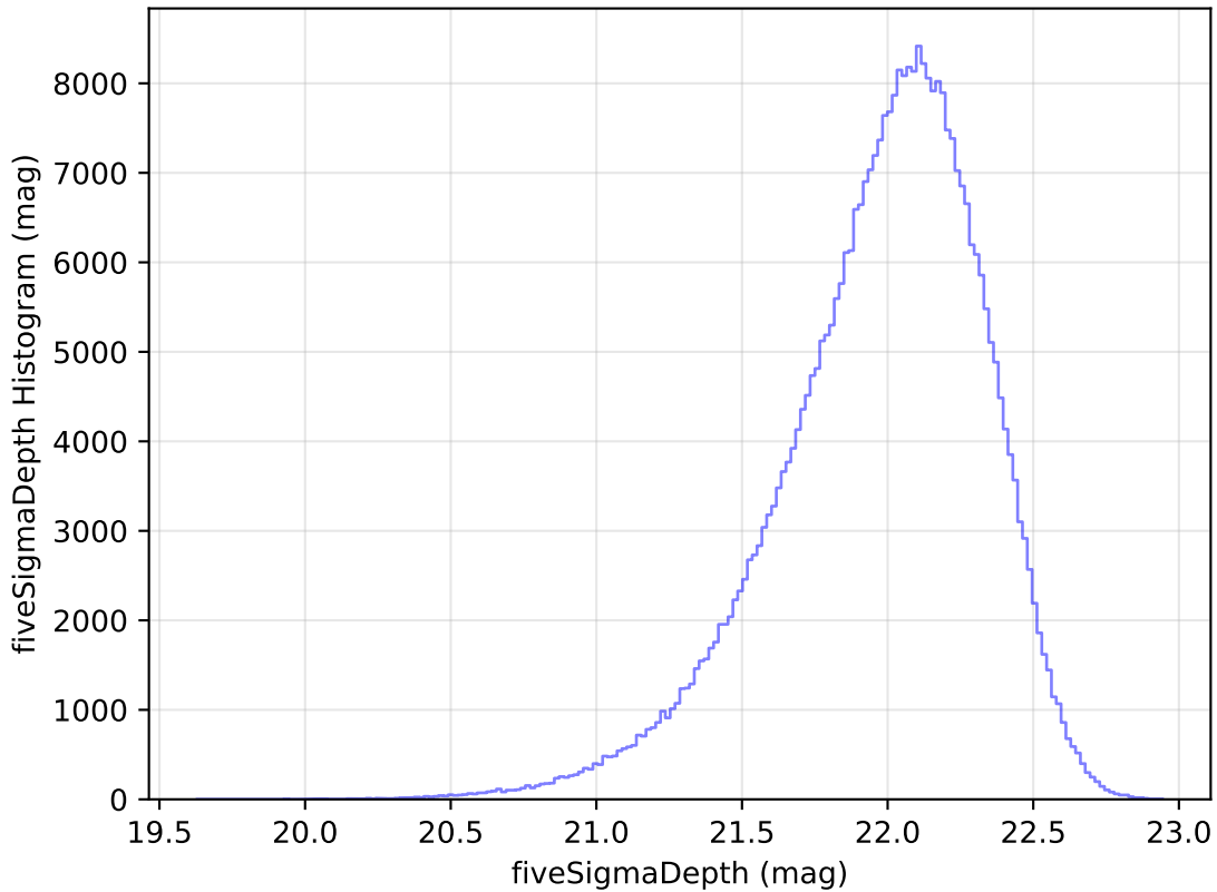
too_elab_r64_d2_giz_v3.4_10yrs All sky y band: fiveSigmaDepth Histogram
