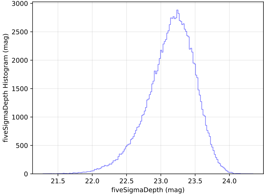
too_elab_r64_d2_giz_v3.4_10yrs All sky u band: fiveSigmaDepth Histogram
