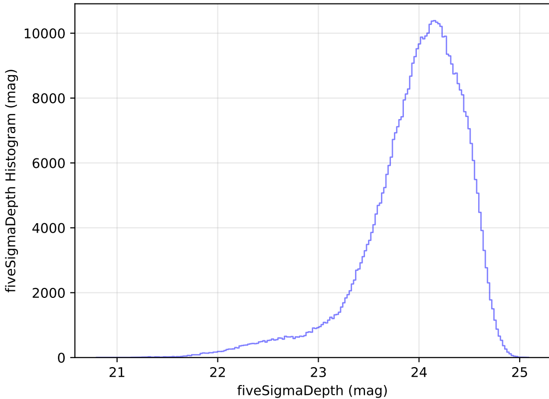
too_elab_r64_d2_giz_v3.4_10yrs All sky r band: fiveSigmaDepth Histogram
