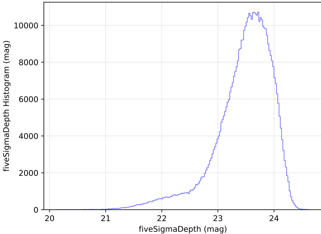
too_elab_r64_d2_giz_v3.4_10yrs All sky i band: fiveSigmaDepth Histogram
