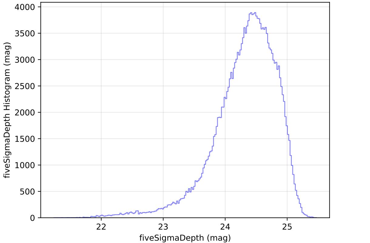
too_elab_r64_d2_giz_v3.4_10yrs All sky g band: fiveSigmaDepth Histogram
