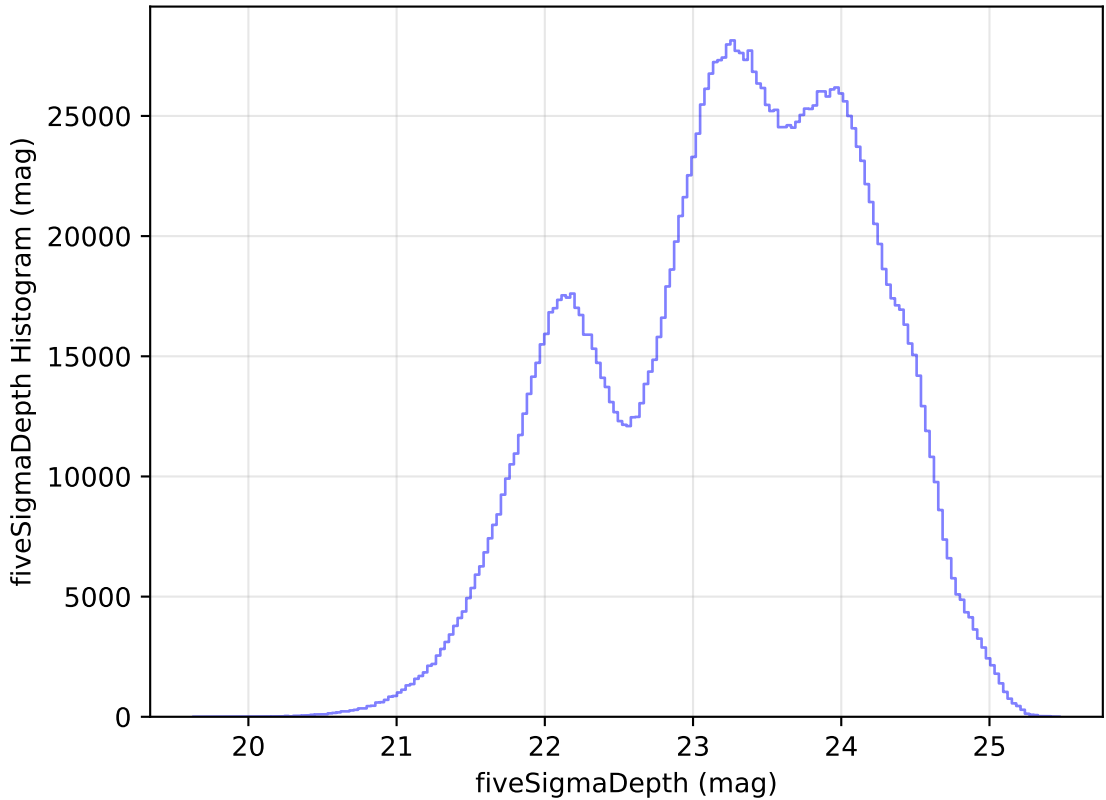
too_elab_r64_d2_giz_v3.4_10yrs All sky all bands: fiveSigmaDepth Histogram
