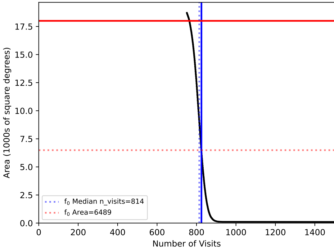
too_elab_r64_d2_giz_v3.4_10yrs WFD: f0
