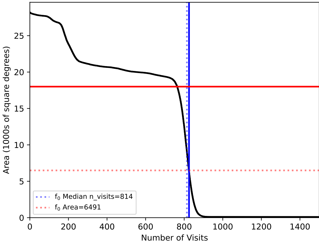
too_elab_r64_d2_giz_v3.4_10yrs All sky: f0
