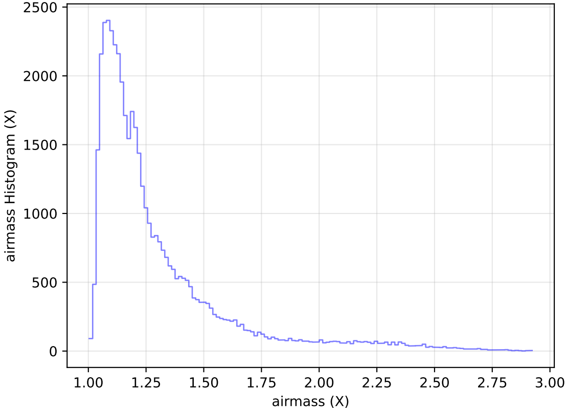
too_elab_r64_d2_giz_v3.4_10yrs Yr 1 z band: airmass Histogram
